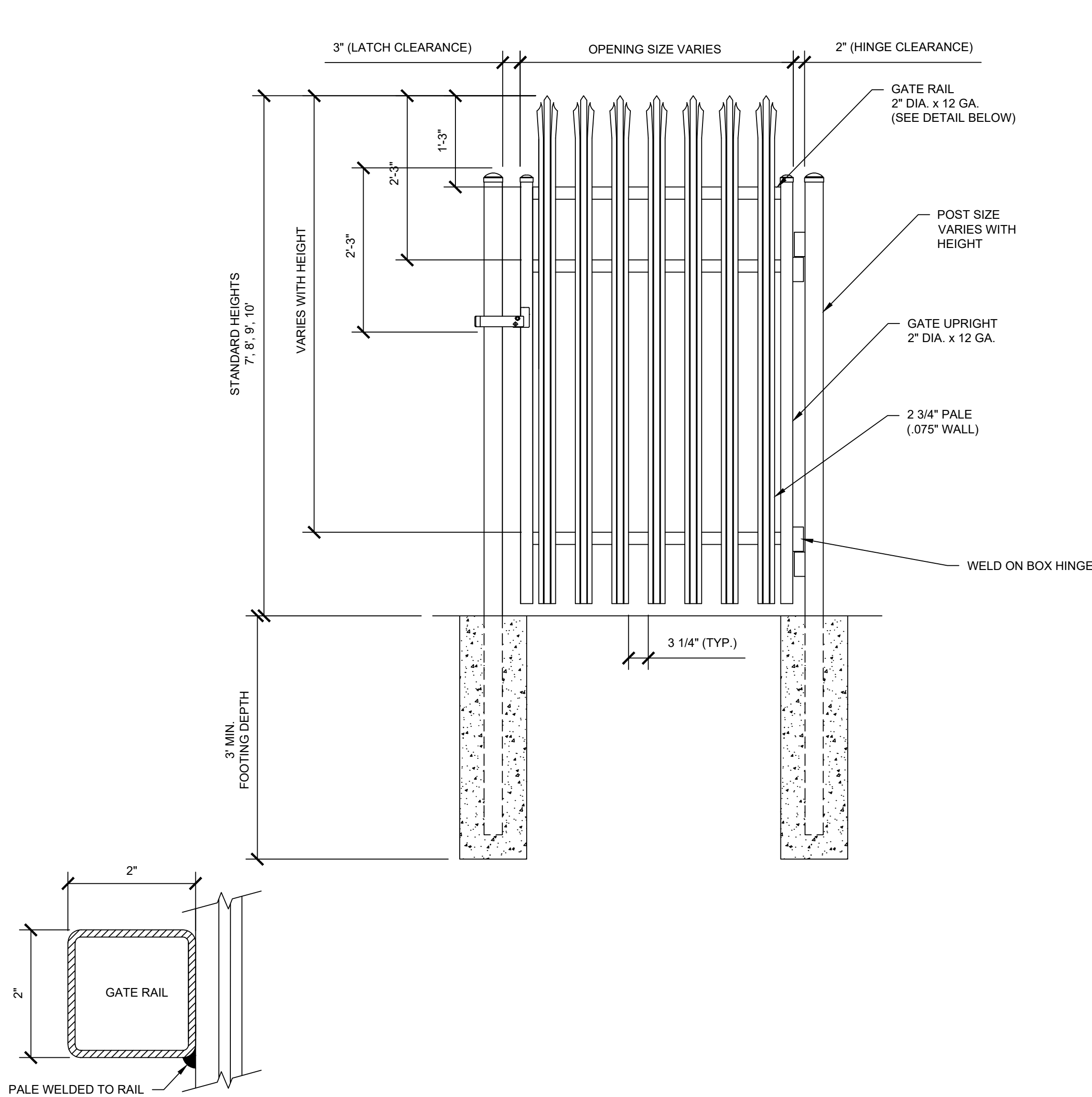
1 DECORATIVE METAL SINGLE SECURITY GATE C601 SCALE: NTS
