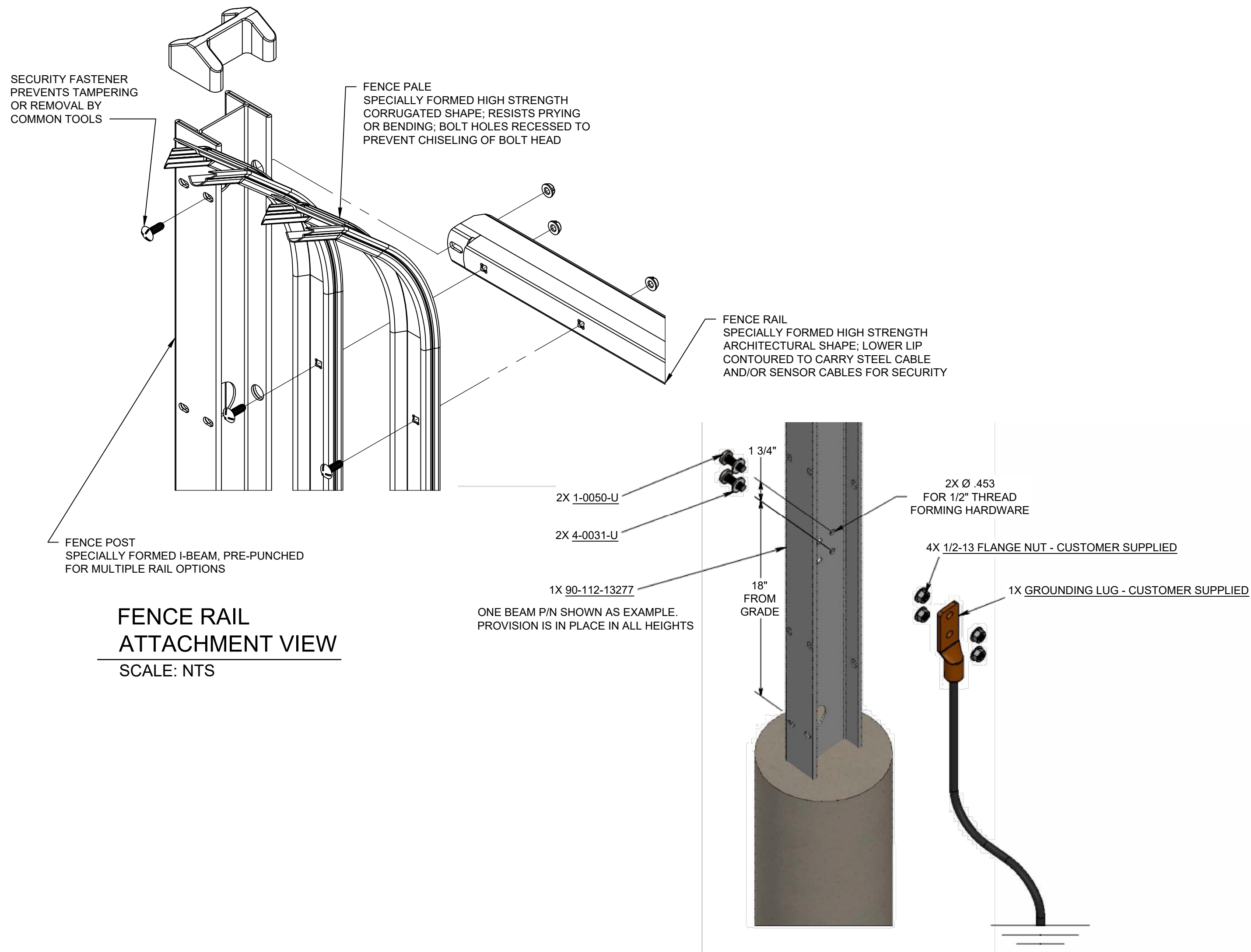
FENCE RAIL SCALE: NTS
