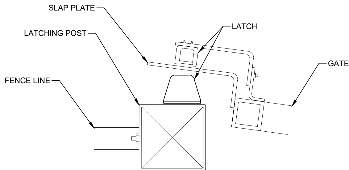
3 SWING GATE LATCH DETAIL C601 SCALE: NTS
